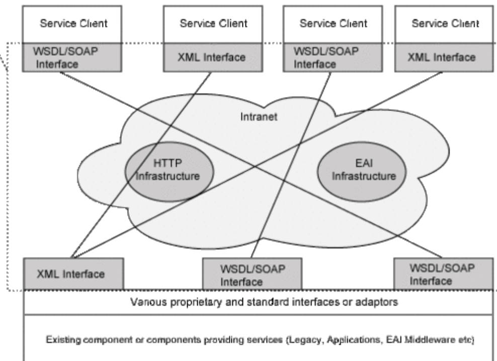
Enterprise Service Bus Components
